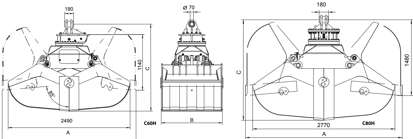
C60H
